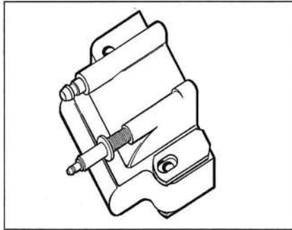
Ignition coil terminal extender CO3010 P/N 502054
